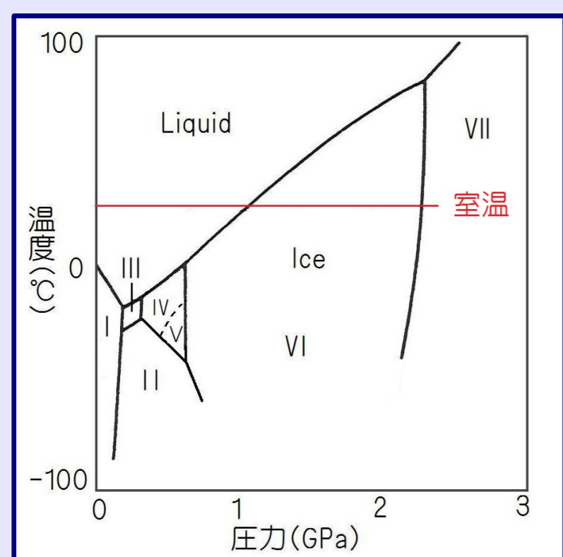
Phase diagram of water
